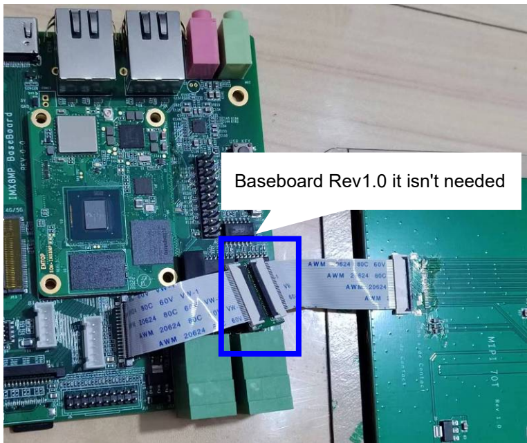
Figure 2-2 MIPI-70T Connection
