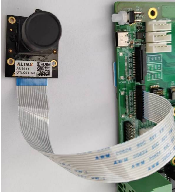
Figure 2-5 AN5641
